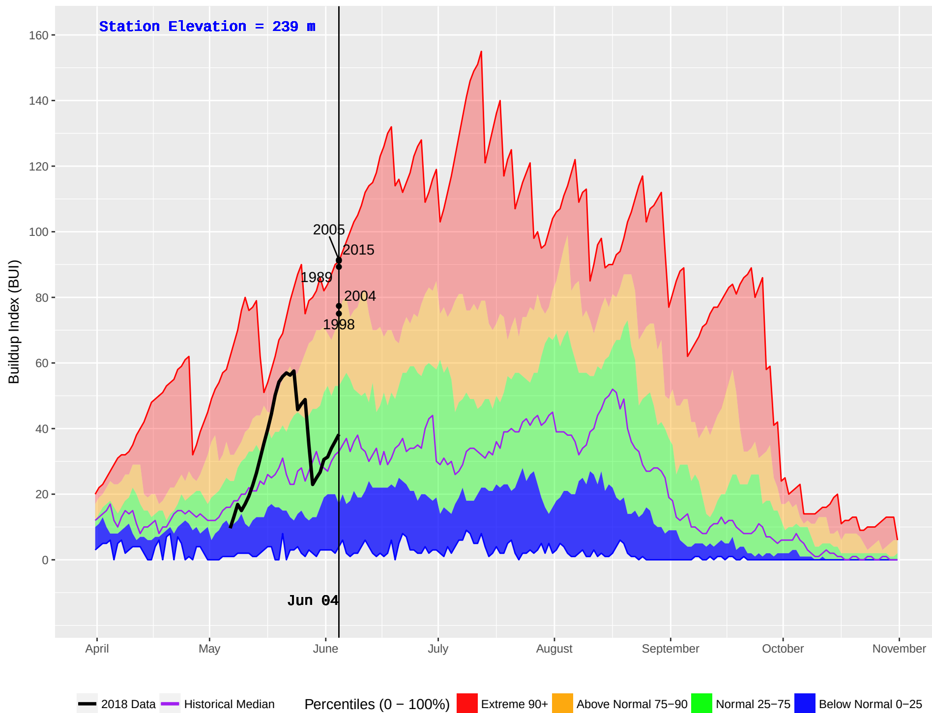
ROSSWOOD (105) : Historical (1970–2016) and Current (2018) Noon Buildup Index (BUI)
